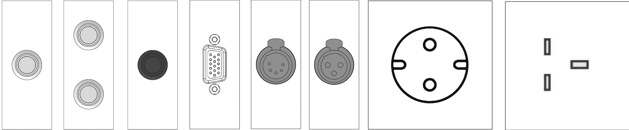
Button (Silver) Dual Button Button (Black) VGA XLR 5-pin XLR 3-pin SCHUKO British Standard
